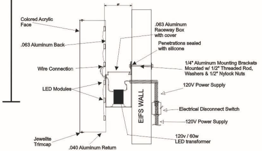
Mounting Detail for Channel Letters on Raceway
