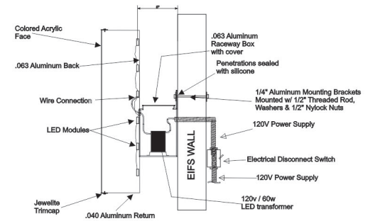
Mounting Detail for Channel Letters on Raceway
