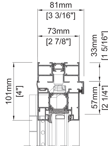
DETAIL 2
