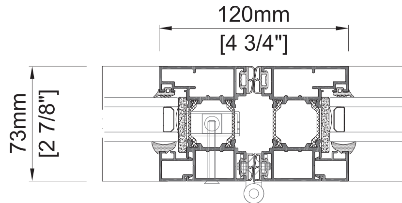
DETAIL 4
