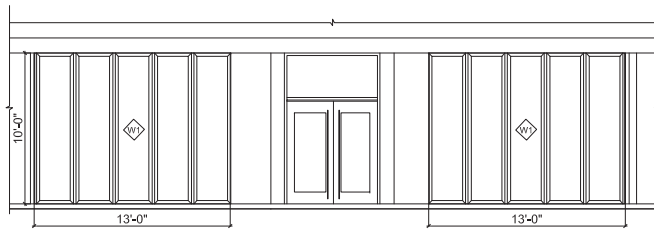
PROPOSED FRONT ELEVATION (EXTERIOR VIEW)
