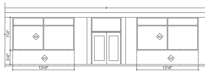
EXISTING INSIDE ELEVATION
