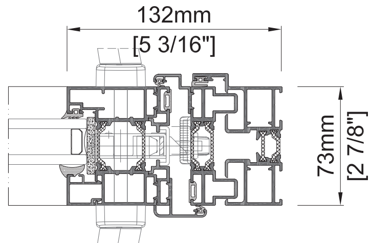
DETAIL 6
