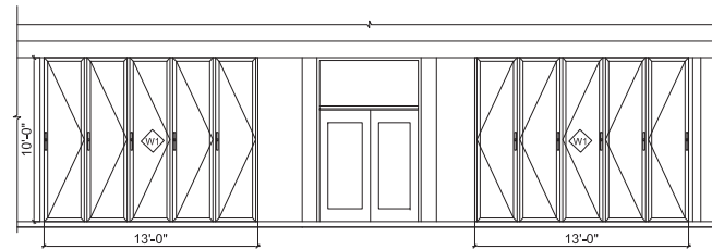
PROPOSED INSIDE ELEVATION
