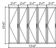
WINDOWS DETAILS-INTERIOR VIEW
