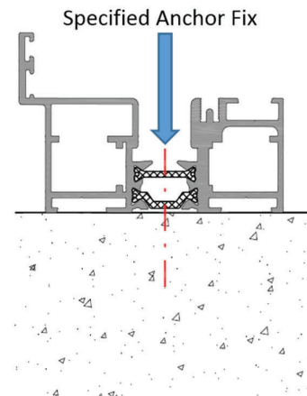
Typical outer frame installation
