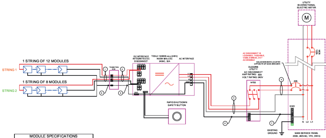
3-LINE DIAGRAM
