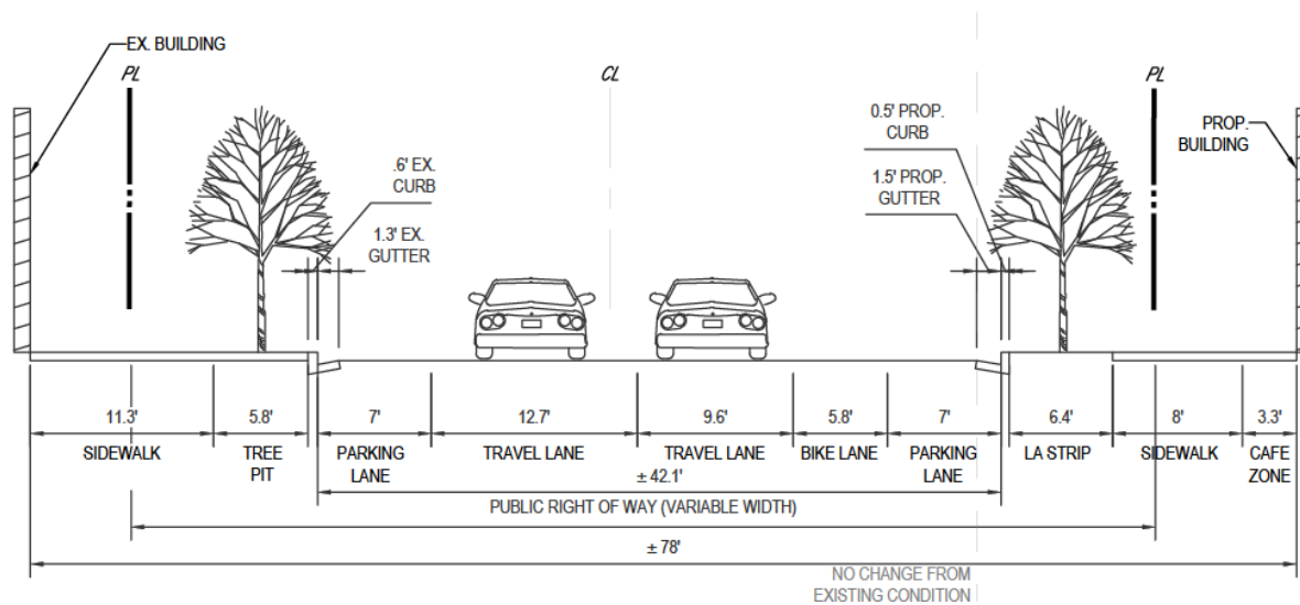
Figure 18 - Proposed Wilson Boulevard Cross Section
