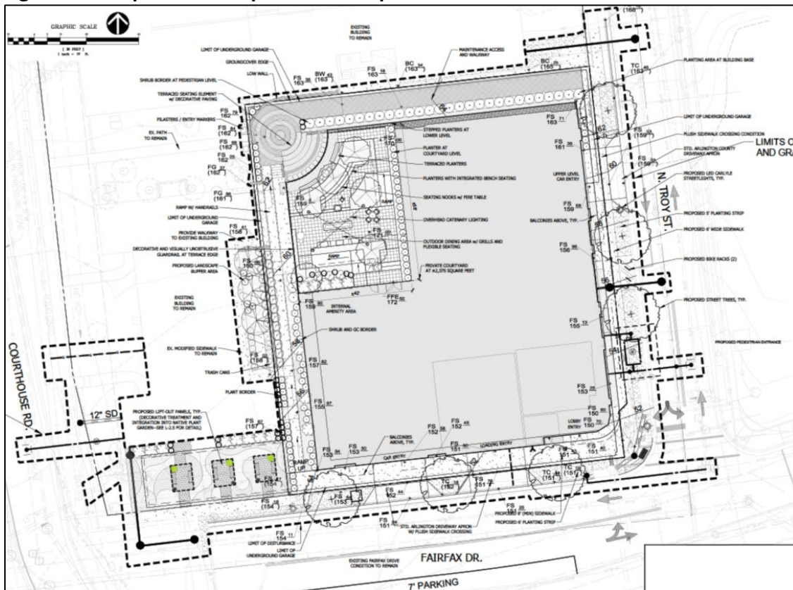
Figure 28. Proposed Conceptual Landscape Plan
