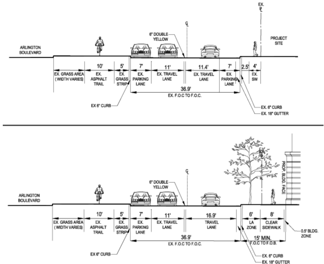
Figure 30. Existing (top) and Proposed (bottom) Fairfax Drive Cross-section
