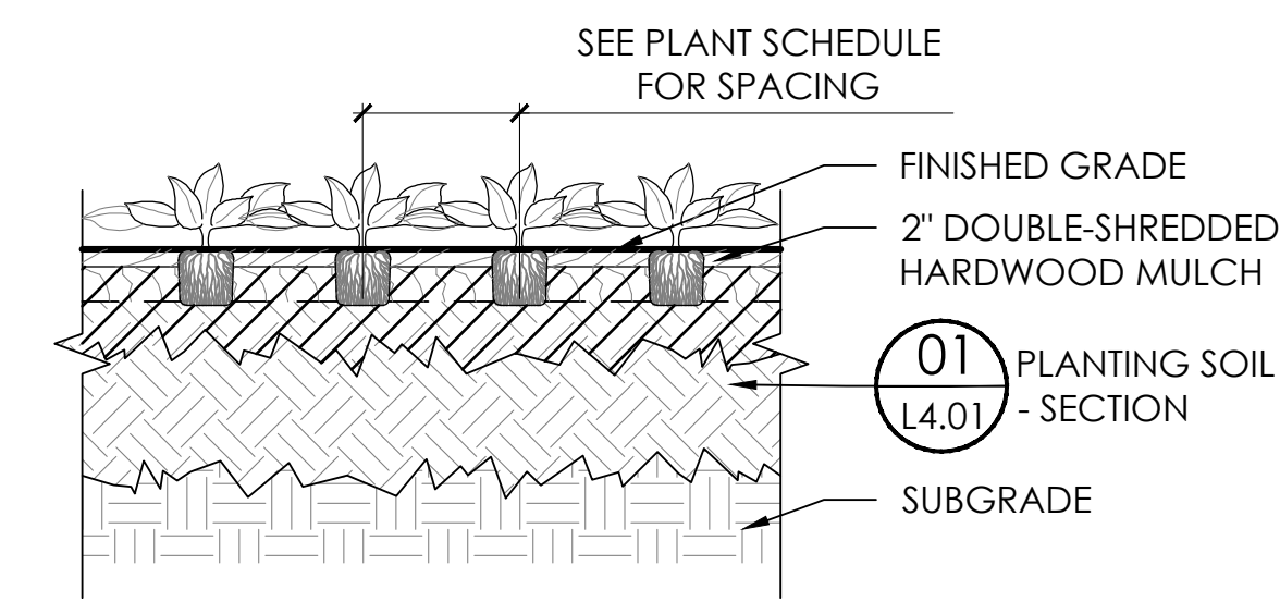
03 PERENNIAL PLANTING - SECTION SCALE: 1/2" = 1'-0"
